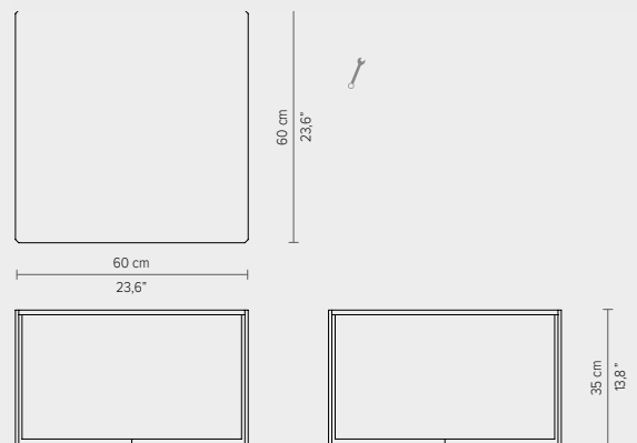
06180 - Coffee table low 60x60cm / 23,50"x23,50"
