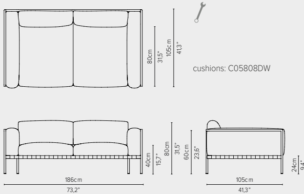
05808D-x - Sofa 2-seater 189 cm
