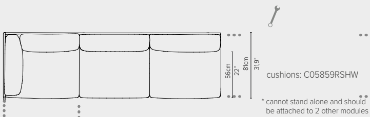
05859RS-x - Right corner extension 273 cm*
