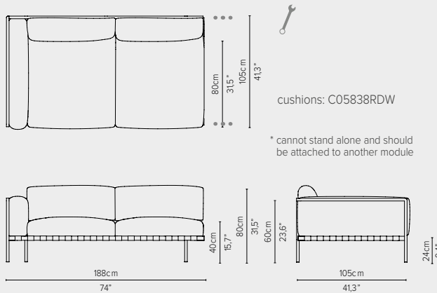
05838RD-x - Right arm extension 189 cm*
